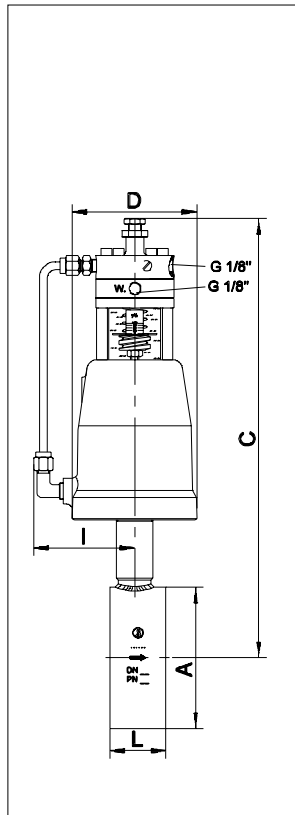
Type 8044 with p/p-positioner Type 8047 with position indicator
