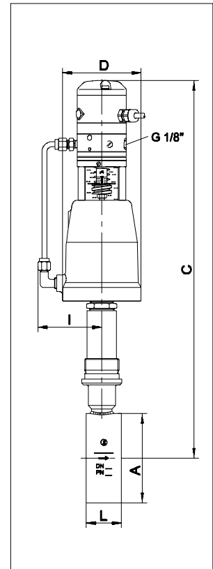
Type 8043 with i/p-positioner Type 8047 with position indicator
