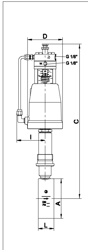
Type 8043 with p/p-positioner Type 8047 with position indicator
