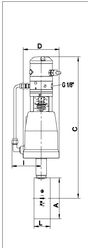
Type 8044 with i/p-positioner Type 8047 with position indicator
